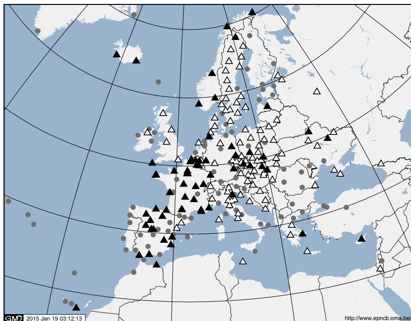
Figure 2: EPN tracking stations capable of tracking L5 indicated with \Delta ; those in addition including L5 in their RINEX v2.11 data are indicated by \blacktriangle (status in December 2014).
