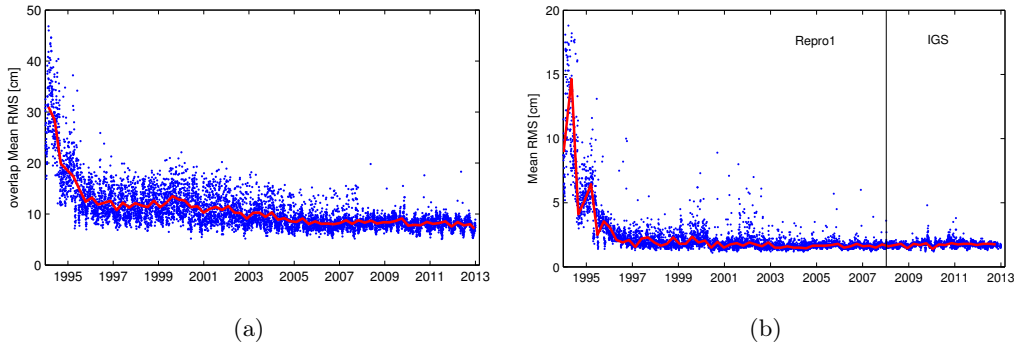
Figure 10: Mean RMS values of IGS processing orbit overlaps (4 hours) [left] and of transformed GFZ IGS reprocessing orbits w.r.t. the reprocessing (1994.0–2008.0) and the IGS Final orbits (2008.0–2013.0) [right]. The solid line represents a 100–day median.
