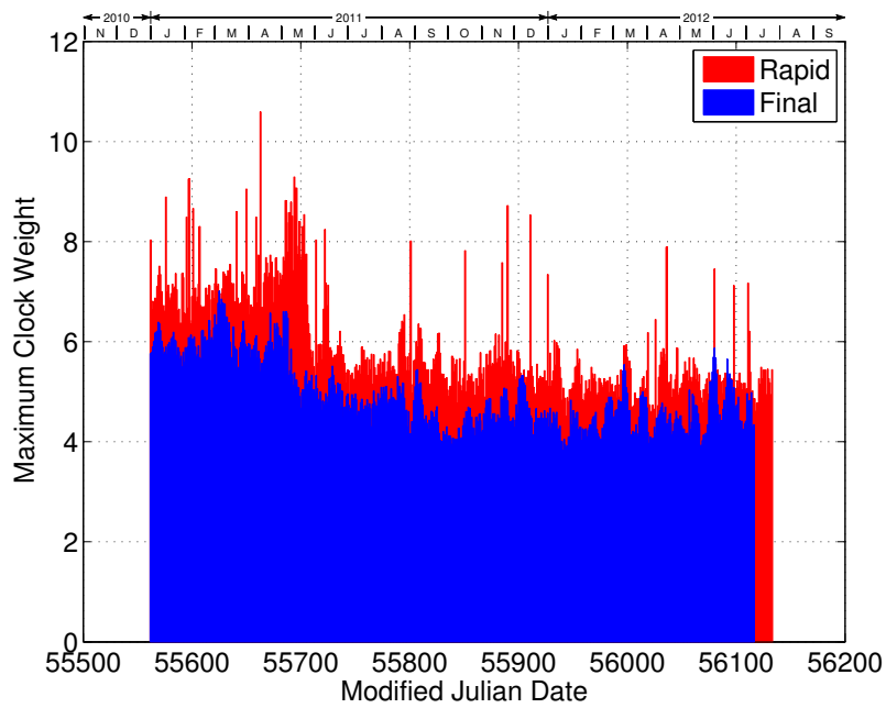
Figure 7: Maximum daily a weight (in %) per clock for the v2.0 IGS Final and Rapid timescales since 2011.
