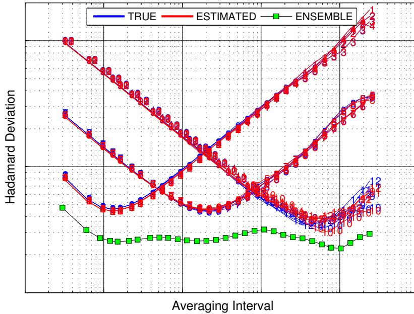
Figure 3: Timescale frequency stability results as measured by the Hadamard deviation statistic for a twelve clock simulation example based on three classes of clocks, where each class is differentiated by a relative different level of RWPH and RWFR noise.
